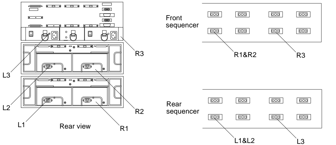
FIGURE 3-13 One StorEdge A3500 Controller Module and Two StorEdge D1000 Disk Arrays (Power)
