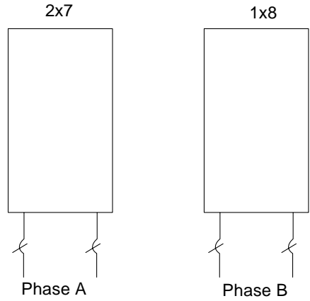
FIGURE 3-23 Power Connections to Avoid (Different Phases)
