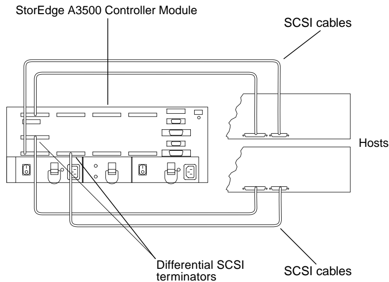
FIGURE 1-4 Two-Node Multi-Host Configuration
