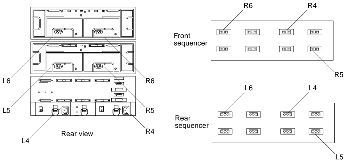
FIGURE 3-14 Two StorEdge D1000 Disk Arrays and One StorEdge A3500 Controller Module (Power)
