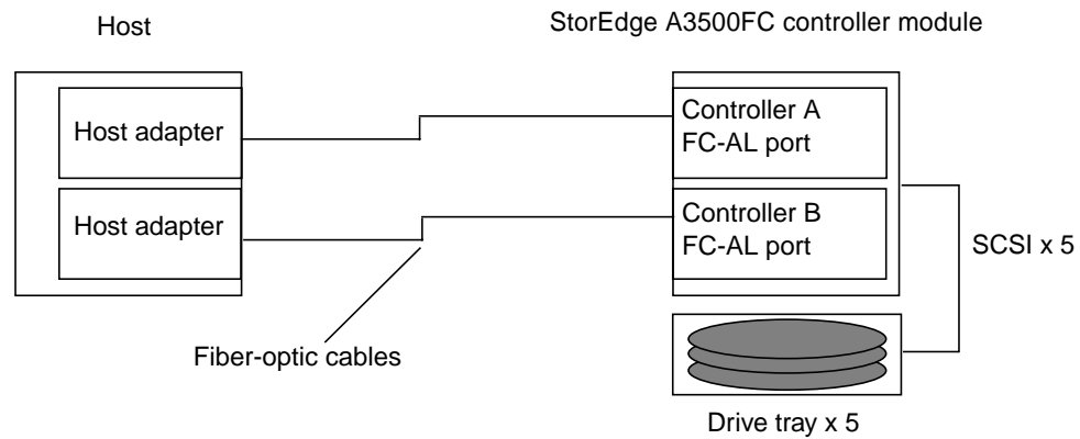
FIGURE 2-2 One Host Connected to One Controller Module
