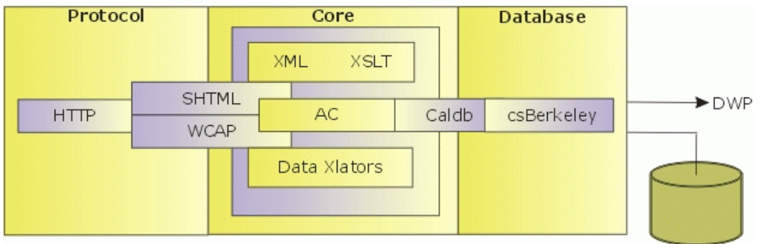
Figure 1-6 Server Architecture
