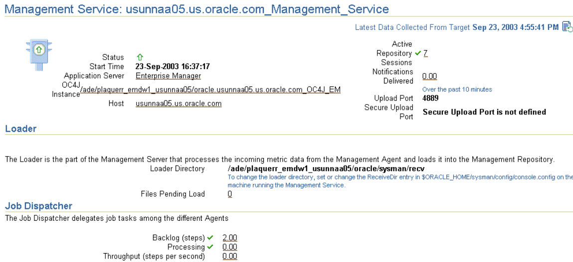
Figure 2–3 Status of an Oracle Management Service
