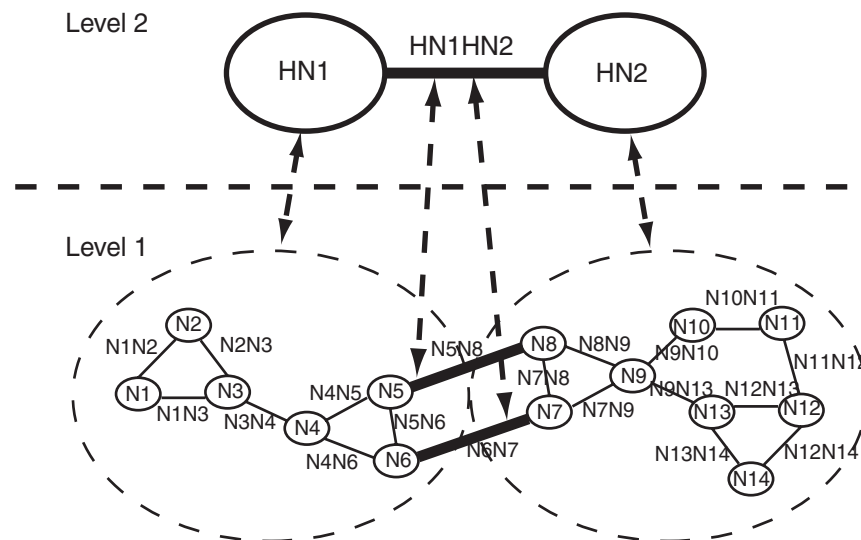
Figure 5-7 Nodes and Links for Logical Network Example
