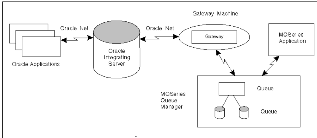
Figure 1-1 Components of the Gateway Architecture
