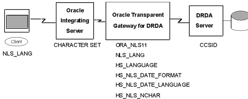
Figure D-1 Architecture of NLS Interactions with Your System Components
