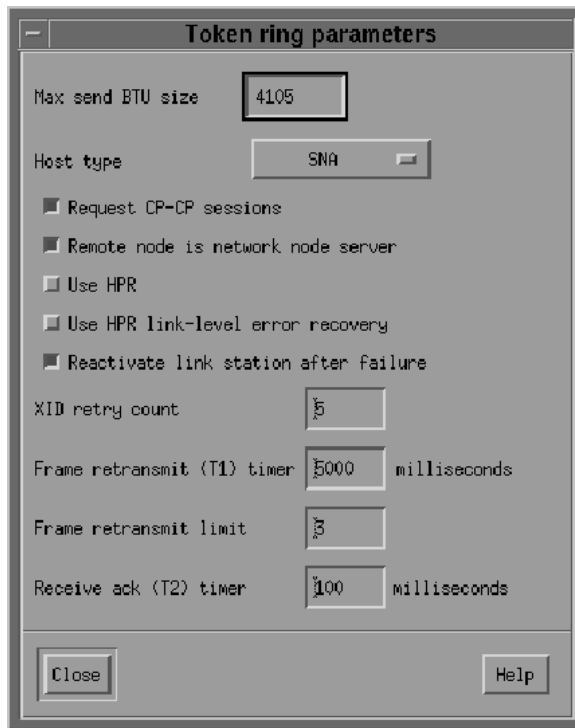
Figure 6–8 Token Ring Parameters Dialog Box
