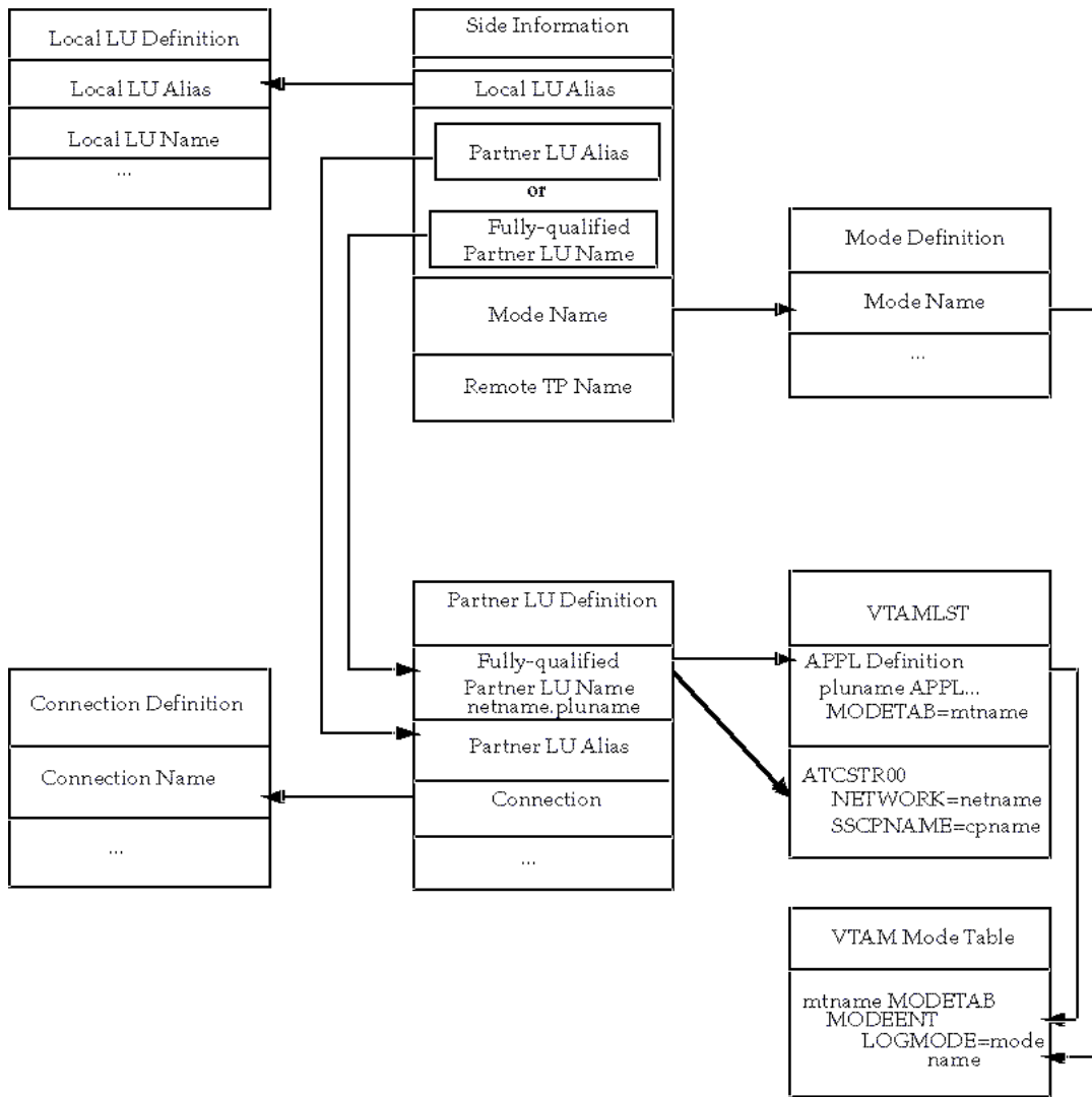
Figure 6–15 Relationship between SNAP-IX Definitions and Host VTAM Definitions
