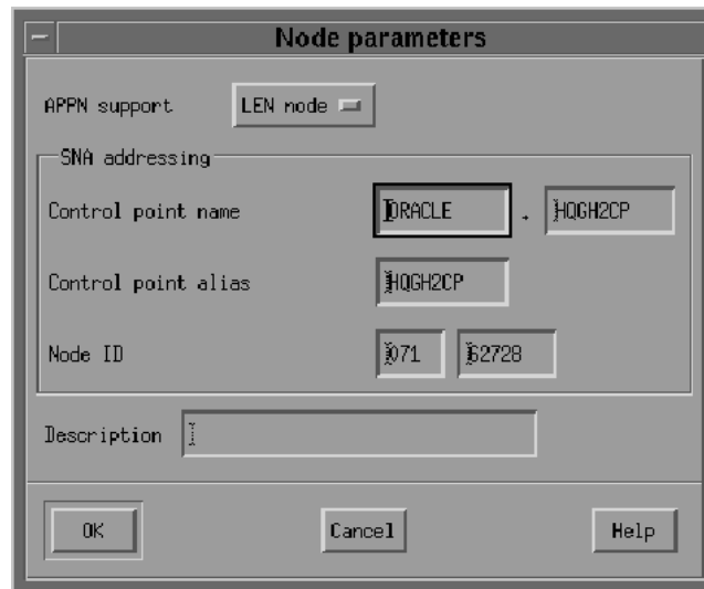
Figure 8–2 Node Parameters Dialog Box
