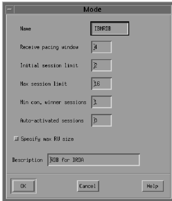
Figure 8–12 IBMRDB Mode Dialog Box
