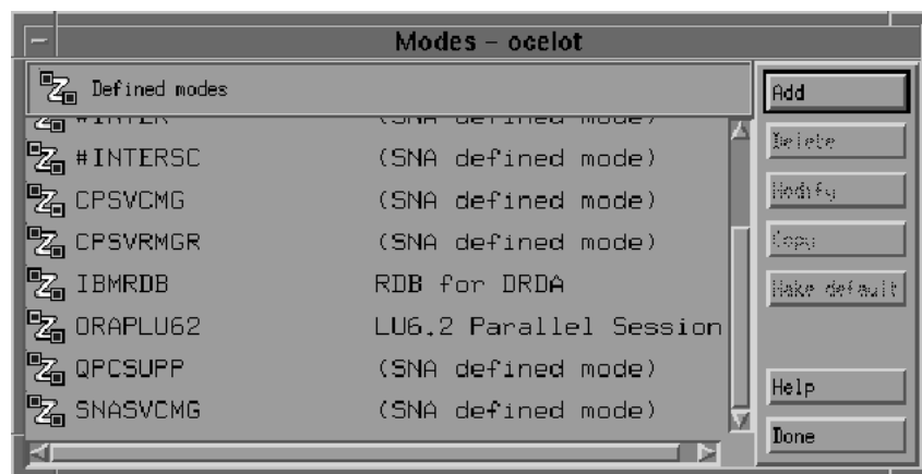
Figure 8–11 Modes Dialog Box
