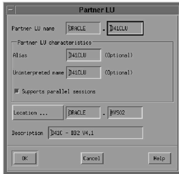
Figure 8–10 Partner LU Dialog Box
