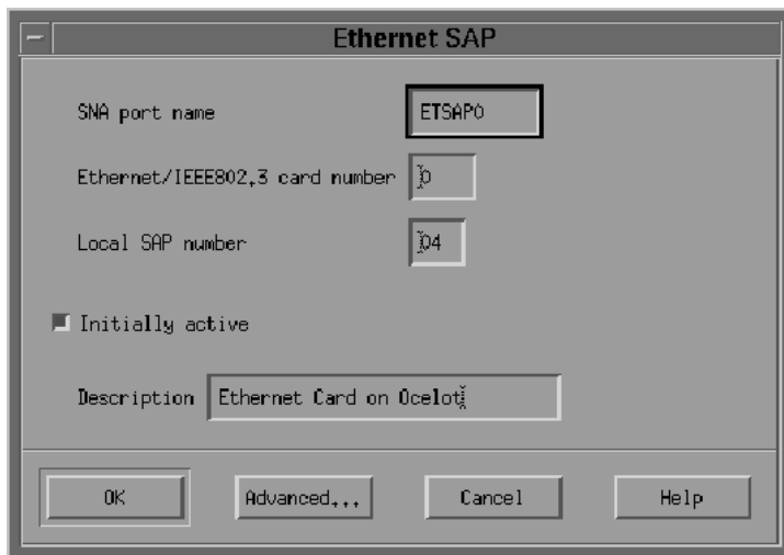
Figure 8–4 Ethernet SAP Dialog Box
