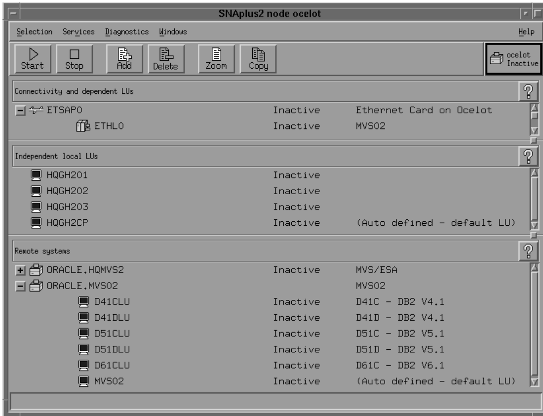
Figure 8–1 xsnapadmin Main Screen
