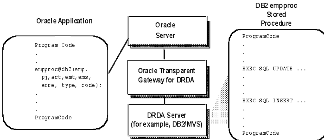
Figure 13–2 Running DRDA Server Stored Procedures
