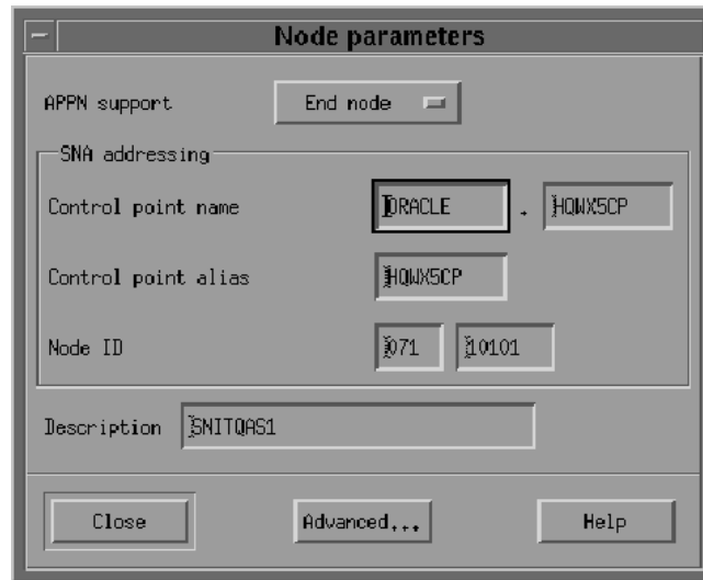
Figure 6–2 Node Parameters Dialog Box
