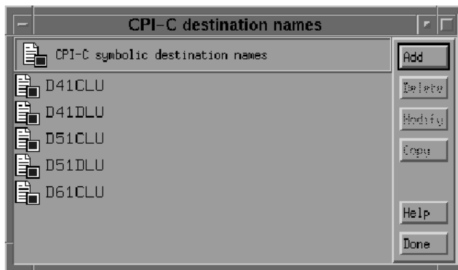
Figure 8–13 CPI-C Destination Names Dialog Box
