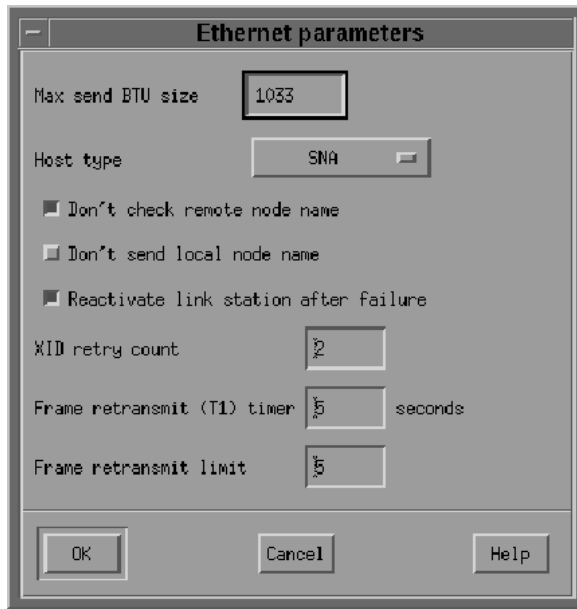
Figure 8–8 Ethernet Parameters Dialog Box
