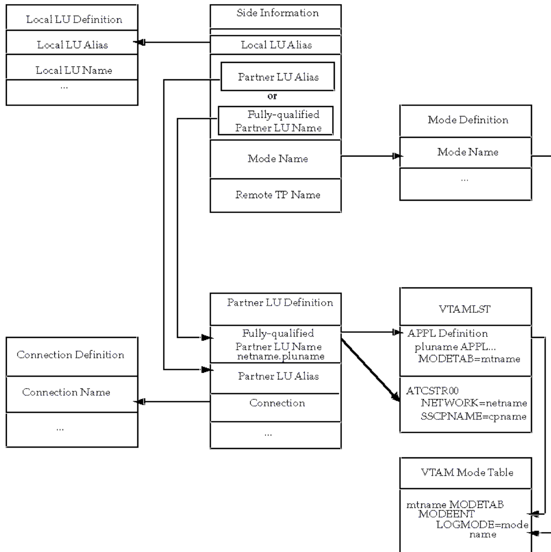
Figure 8-15 Relationship between SNAPPlus2 Definitions and Host VTAM Definitions
