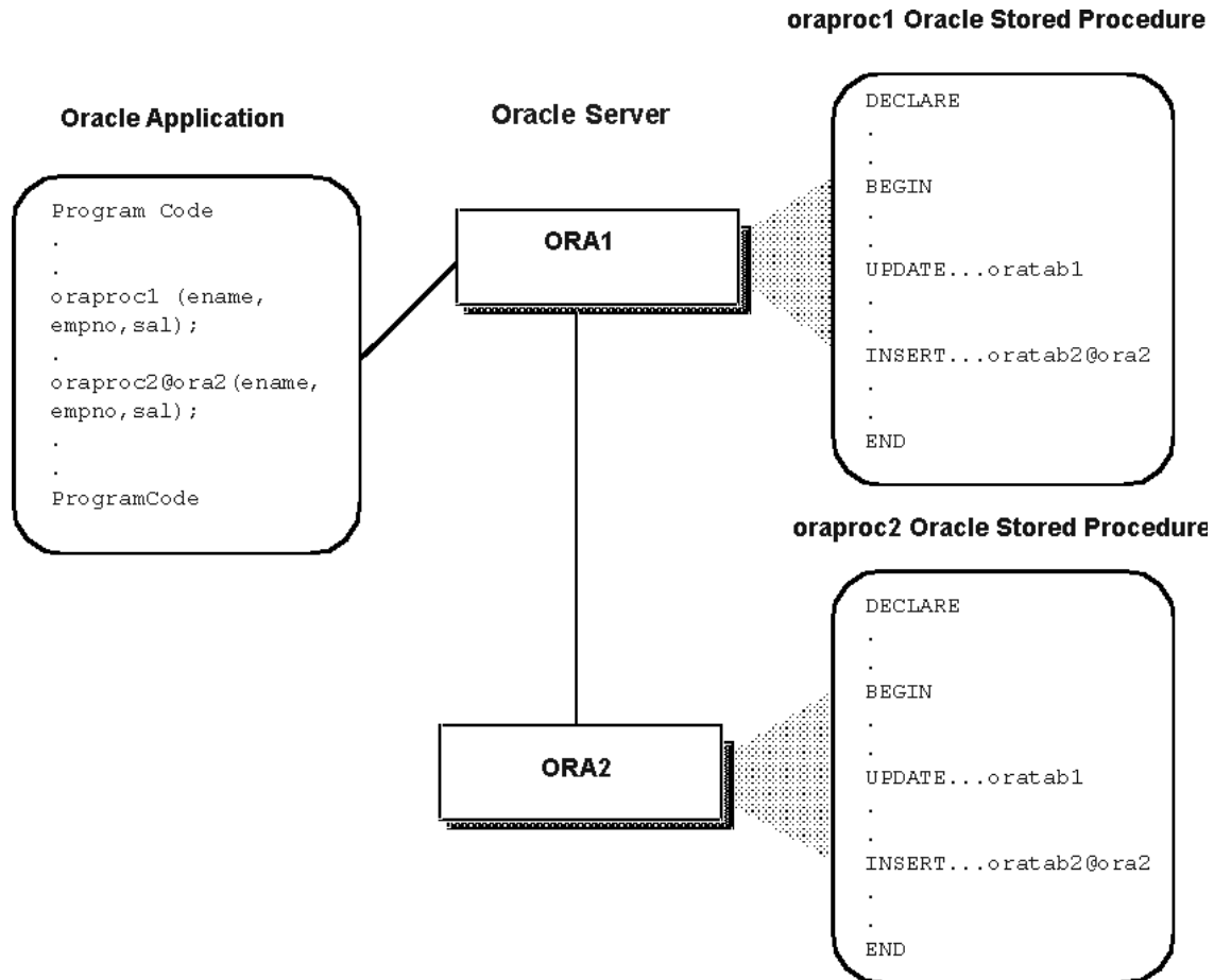
Figure 13–1 Calling Oracle Stored Procedures in a Distributed Oracle Environment
