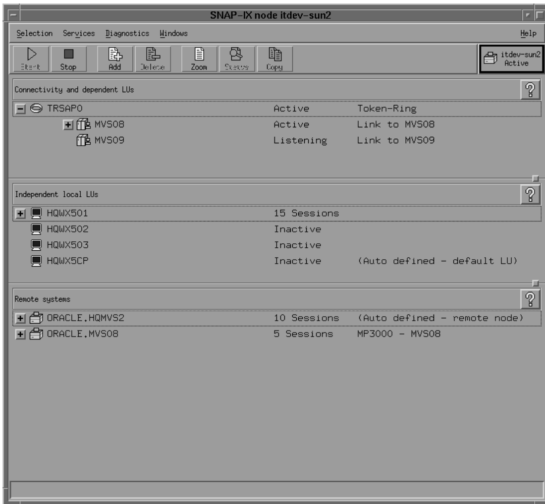
Figure 6-1 xsnaadmin Main Screen
