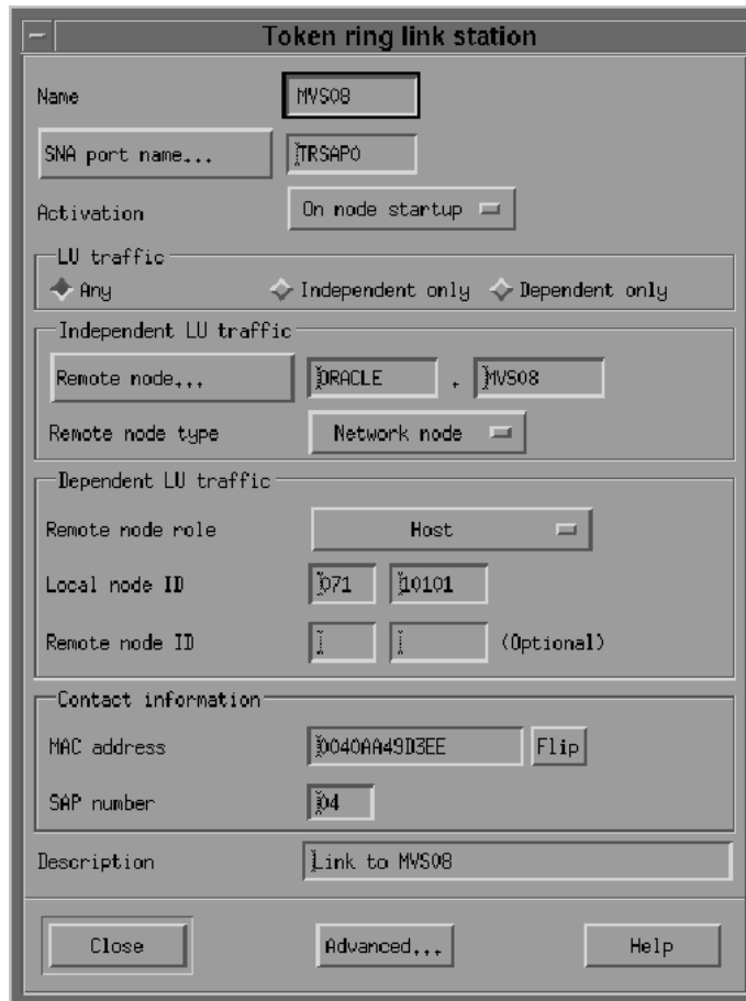
Figure 6–7 Link Station Dialog Box
