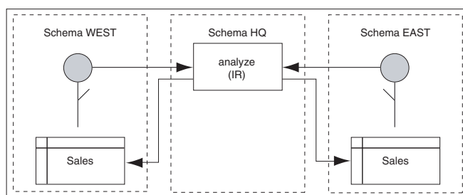
Figure 2-4 Invoker-Rights Solution
