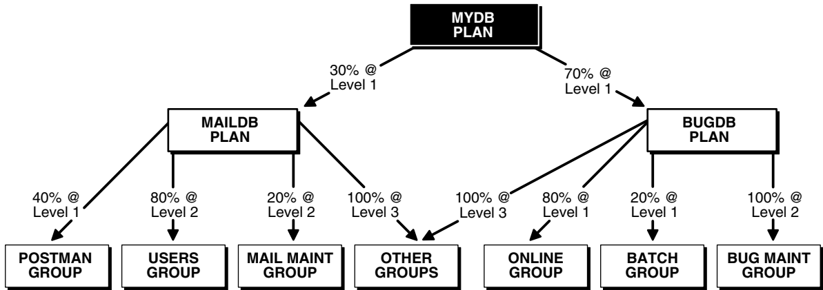
Figure 24–3 Multilevel Schema
