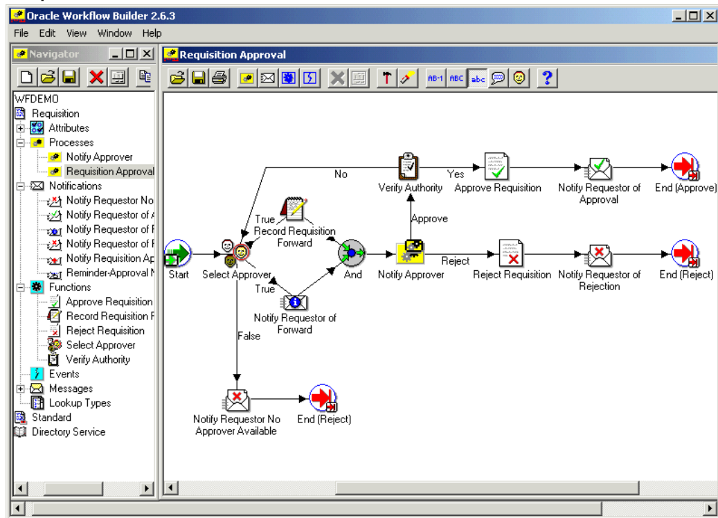
Sample Workflow Process in Oracle Workflow Builder
