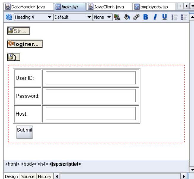
Figure 4–11 Login Page
