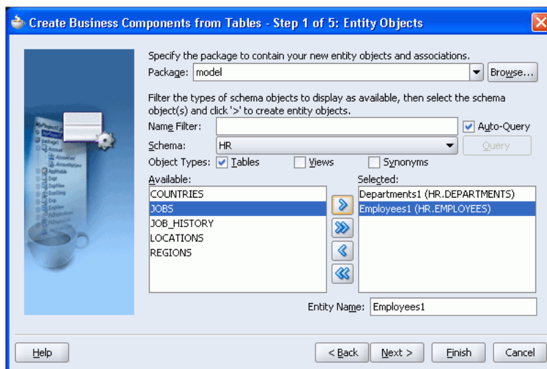
Figure 7–2 Selecting Schema Objects to Create Entity Objects
