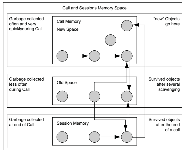
Figure 1–6 Garbage Collection
