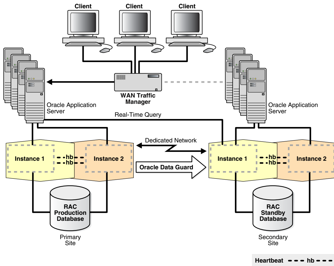
Figure 4–9 Oracle Database with Oracle RAC and Data Guard - MAA
