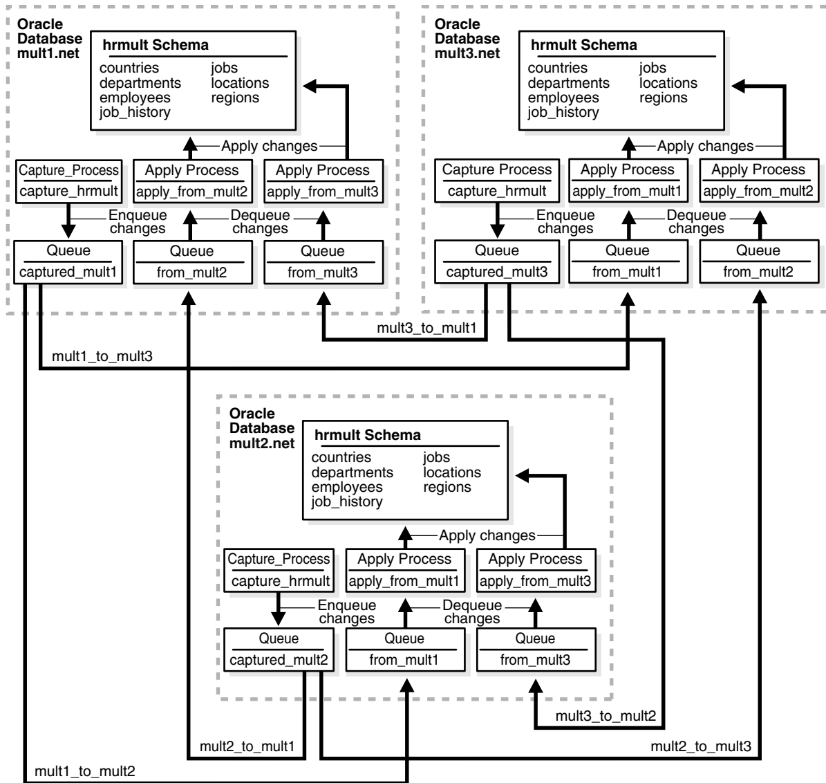
Figure 4–10 Oracle Database with Streams Architecture That Shares Data From Multiple Databases
