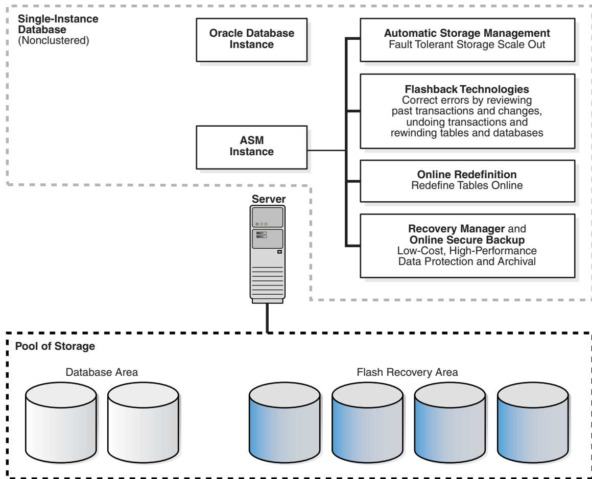
Figure 4–1 Single-Node, Nonclustered Oracle Database with an ASM Instance
