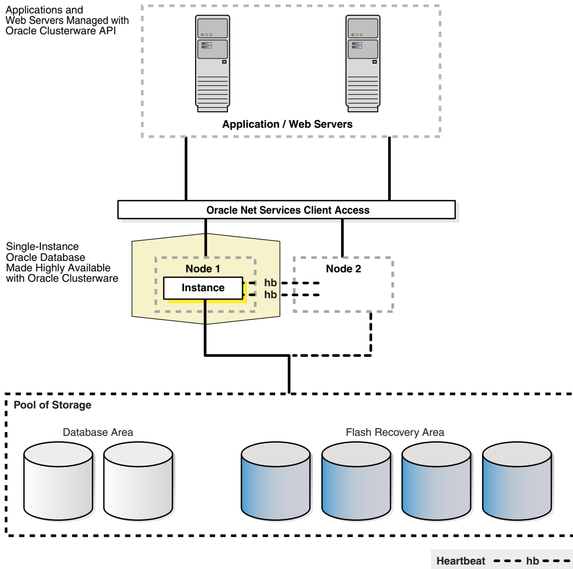
Figure 4–2 Oracle Database with Oracle Clusterware (Before Cold Cluster Failover)
