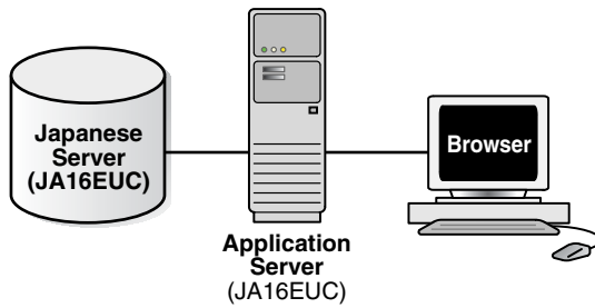
Figure 2–4 Multitier Monolingual Database Scenario
