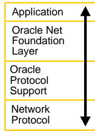
Figure 1–18 Oracle Net on the Client
