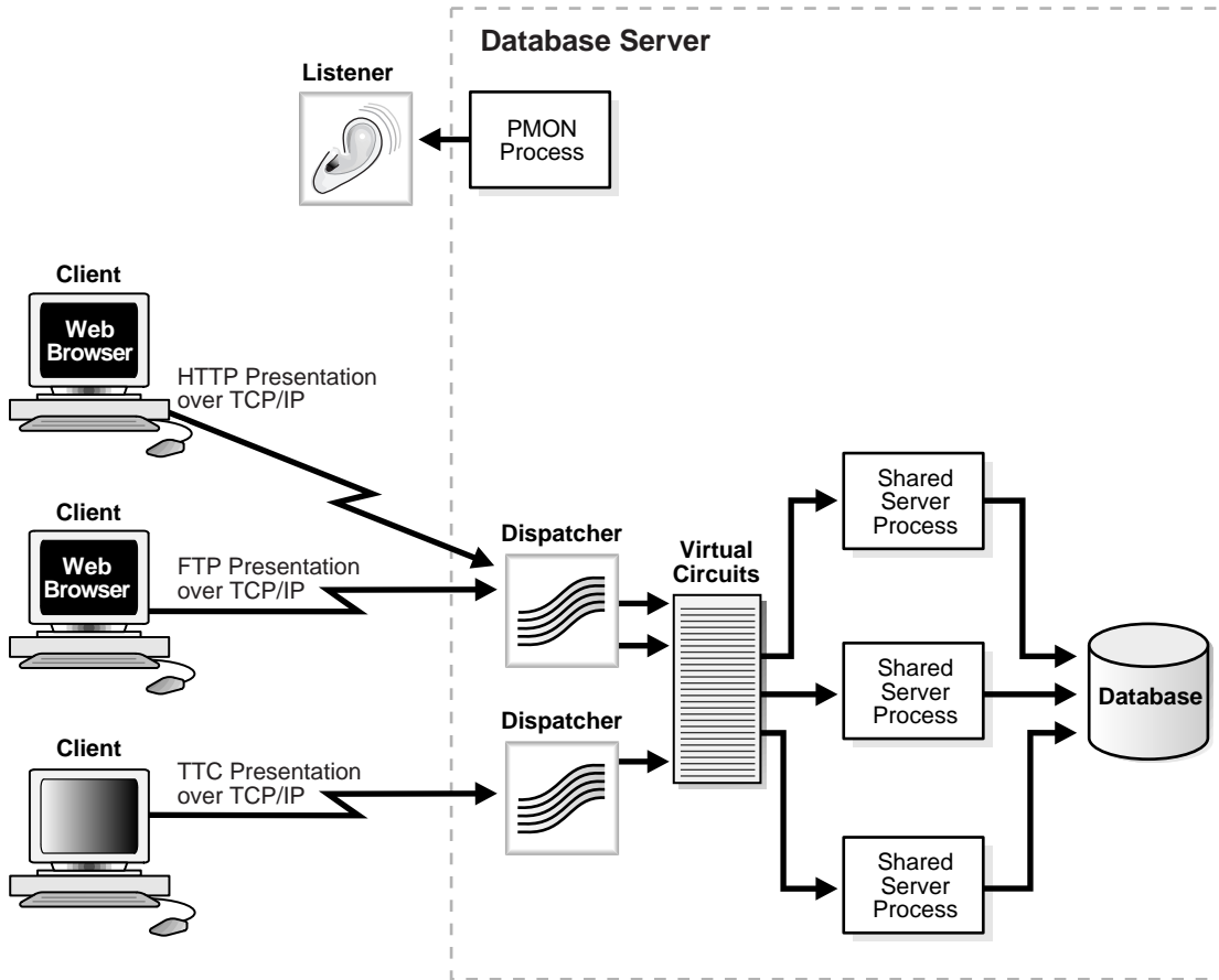
Figure 4-8 Shared Server Architecture
