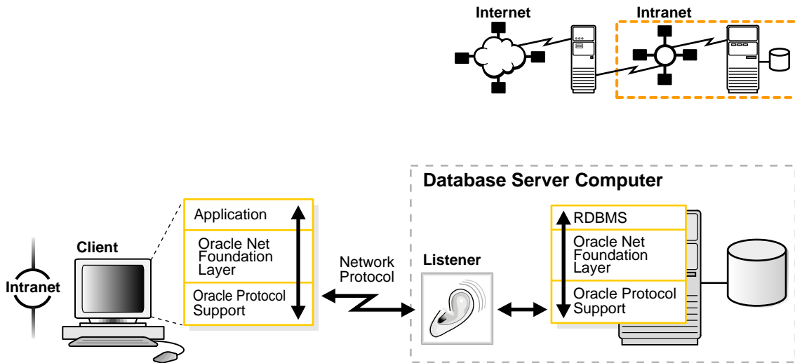
Figure 1-20 Listener in a Connection Request
