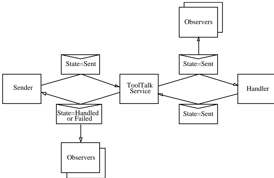
FIGURE 8-2 Request Routing
