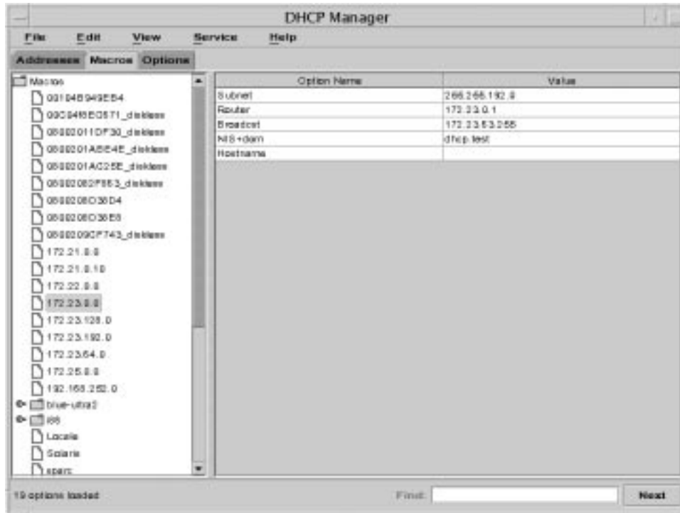
Figure 4-6 DHCP Manager's Macros Tab
