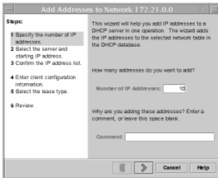
Figure 4-9 Address Wizard
