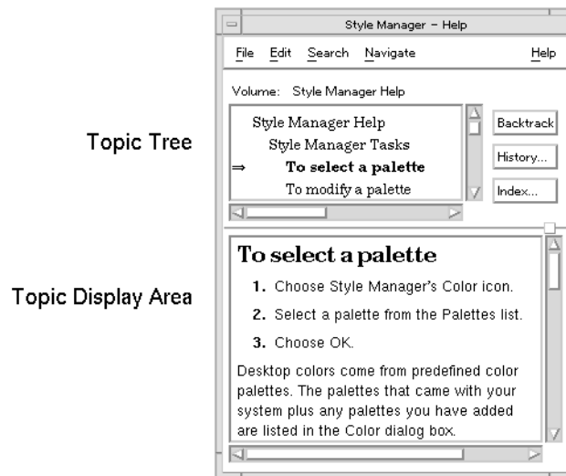
FIGURE 9-1 General help dialog
