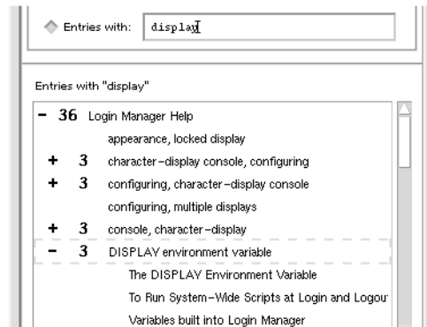
FIGURE 1-7 Index entry prefix notation
