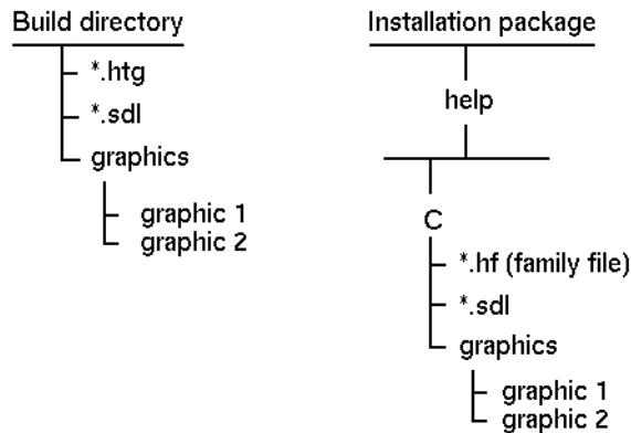
FIGURE 13-2 Relationship of build directories and installation package
