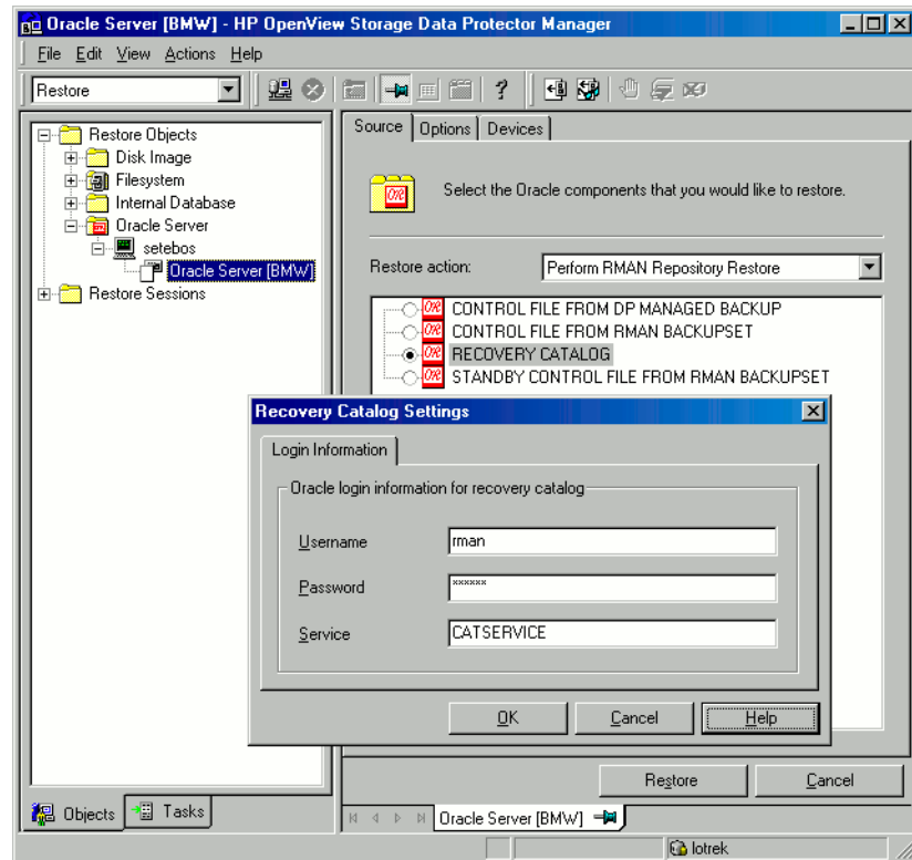
Figure 1-18 Recovery Catalog and Recovery Catalog Settings Dialog Box
