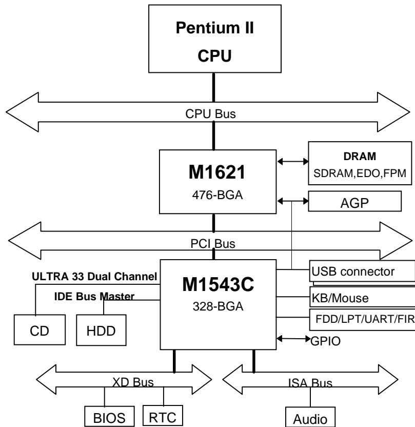
Figure 1.2 Aladdin Pro II System Block Diagram with M1543C
