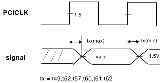
Fig. 7 : Valid Delay Timings
