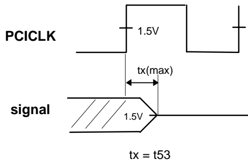
Fig. 8 : Float Delay Timings
